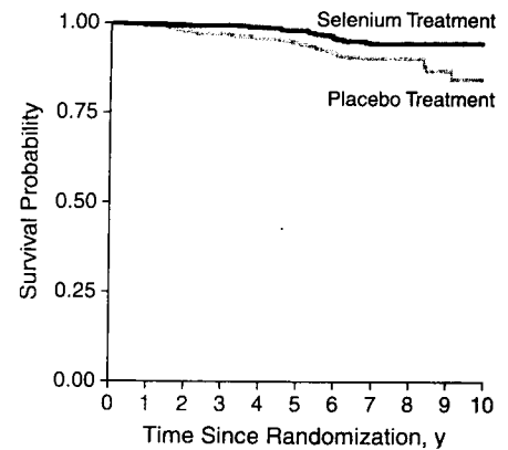
Figure 3.—Kaplan-Meier curve of total cancer mortality.
